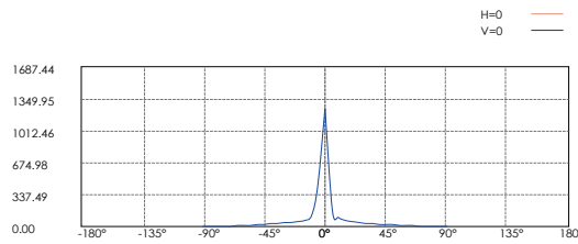
Lux distance Curve
