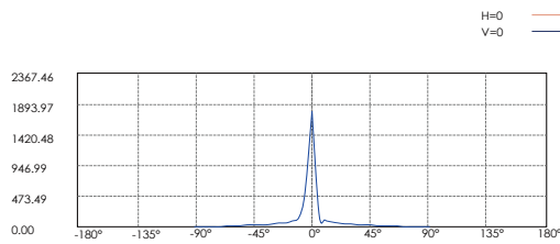
Lux distance Curve
